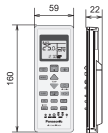
<Remote Control>
